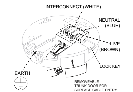
FIGURE 5 – WIRING & INTERCONNECT FACILITY
