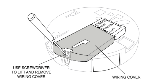
FIGURE 6 – REMOVE WIRING COVER
