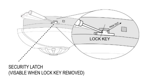
FIGURE 8 – USE SCREW TO PICK OUT THE LOCK KEY FROM THE MOUNTING BASE
